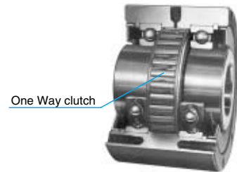
One Way clutch (Package Type)
