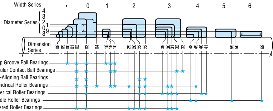
Fig. 3.1 Dimension Series of Radial Bearings
