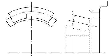
Fig. 14.11 Removal Notches
