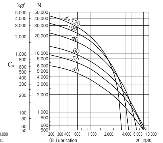
Fig. 5.13 Permissible Axial Load for Cylindrical Roller Bearings For Diameter Series 3 bearings ( k=1.0 ) operating under a continuous load and lubricated with grease or oil.
