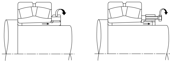
Fig. 14.16 Removal of Withdrawal Sleeve Using Withdrawal Nut (1)
